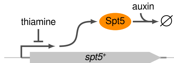
Figure 3.1: Diagram of the dual-shutoff system used to deplete Spt5 from S. pombe . Spt5 is expressed from a thiamine-repressible promoter, and tagged with an auxin-inducible degron tag for specific degradation upon addition of auxin.
